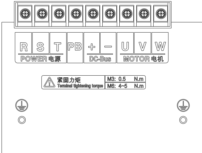
d) GS750-030-3/3B~GS750-037-3/3B
