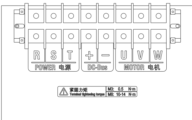
e) GS750-045-3~GS750-110-3
