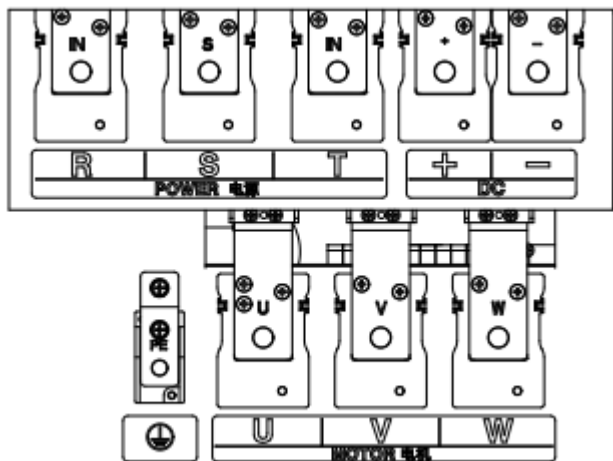
(g) GS750-185-3~GS750-250-3
