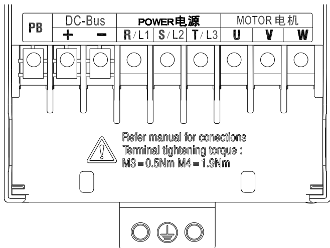
b) GS750-2R2-3B~GS750-4R0-3B
